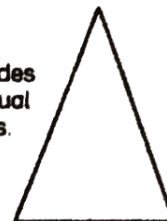
isosceles triangle
