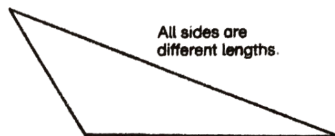
scalene triangle
