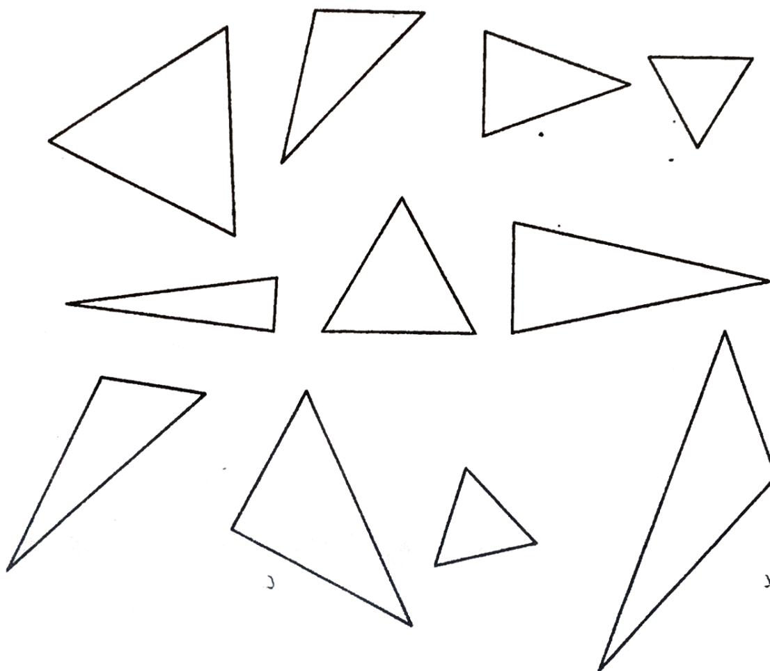
scalene triangle
